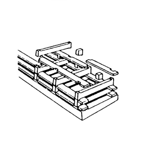
16 The Ebensee Krainer wall → 6 + 13
